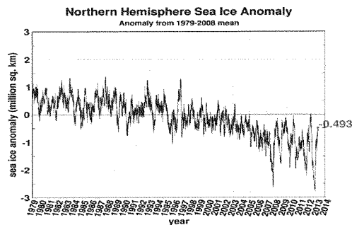
Figure 2. Northern Hemisphere sea ice anomalies http://arctic.atmos.uiuc.edu/cryosphere/IMAGES/seaice.anomaly.arctic.png
