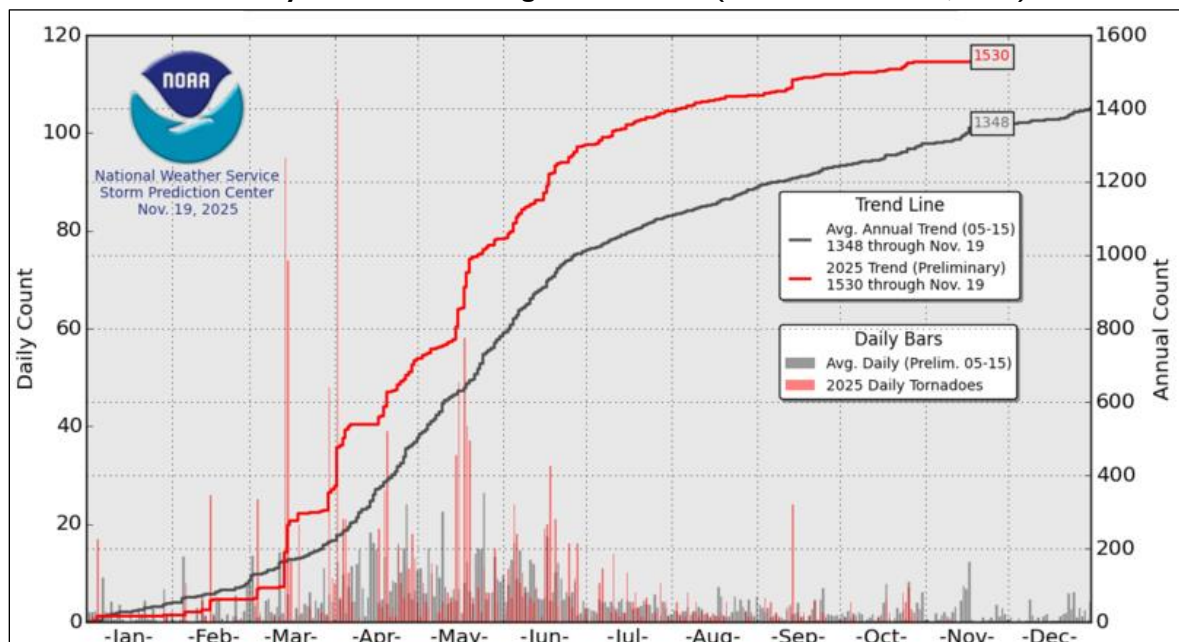
Figure 1. U.S. Tornadoes Daily Count and Running Annual Trend (as of November 19, 2025)
