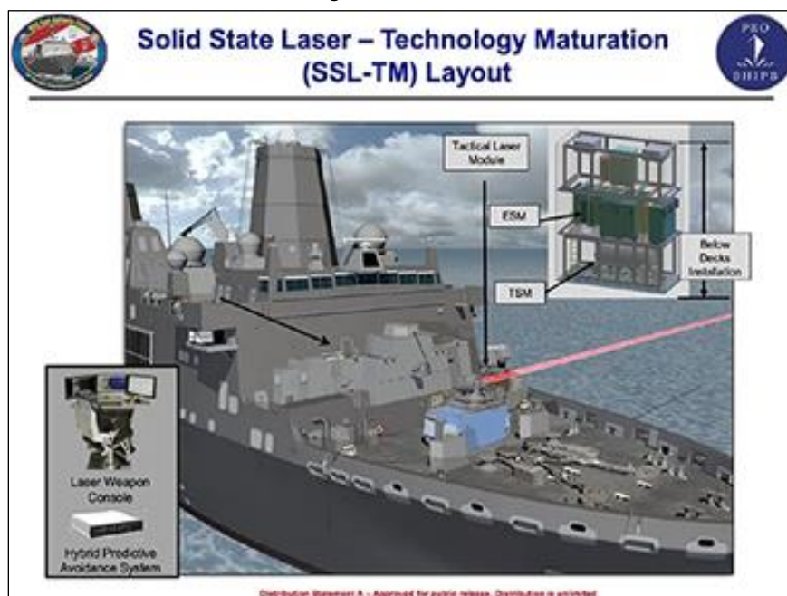
Figure 6. Navy Graphic of SSL-TM Laser System
