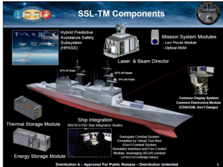
Figure 4. ONR Graphic of SSL-TM Laser System Artist's rendering of installation on Navy's Self Defense Test Ship
