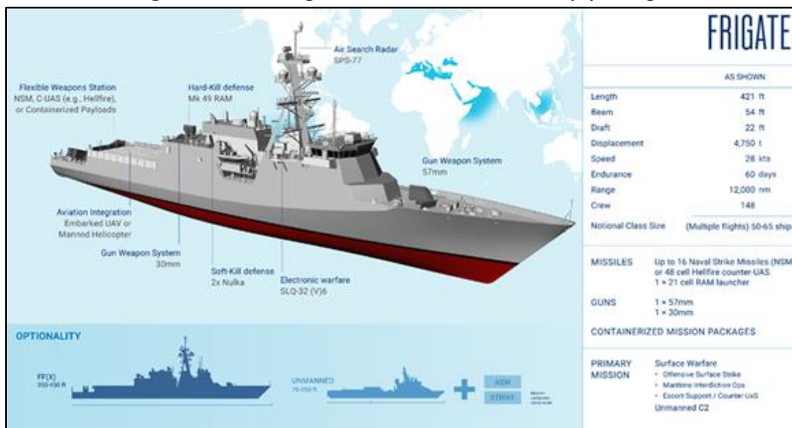
Figure 6. Rendering and Selected Details of FF(X) Design
