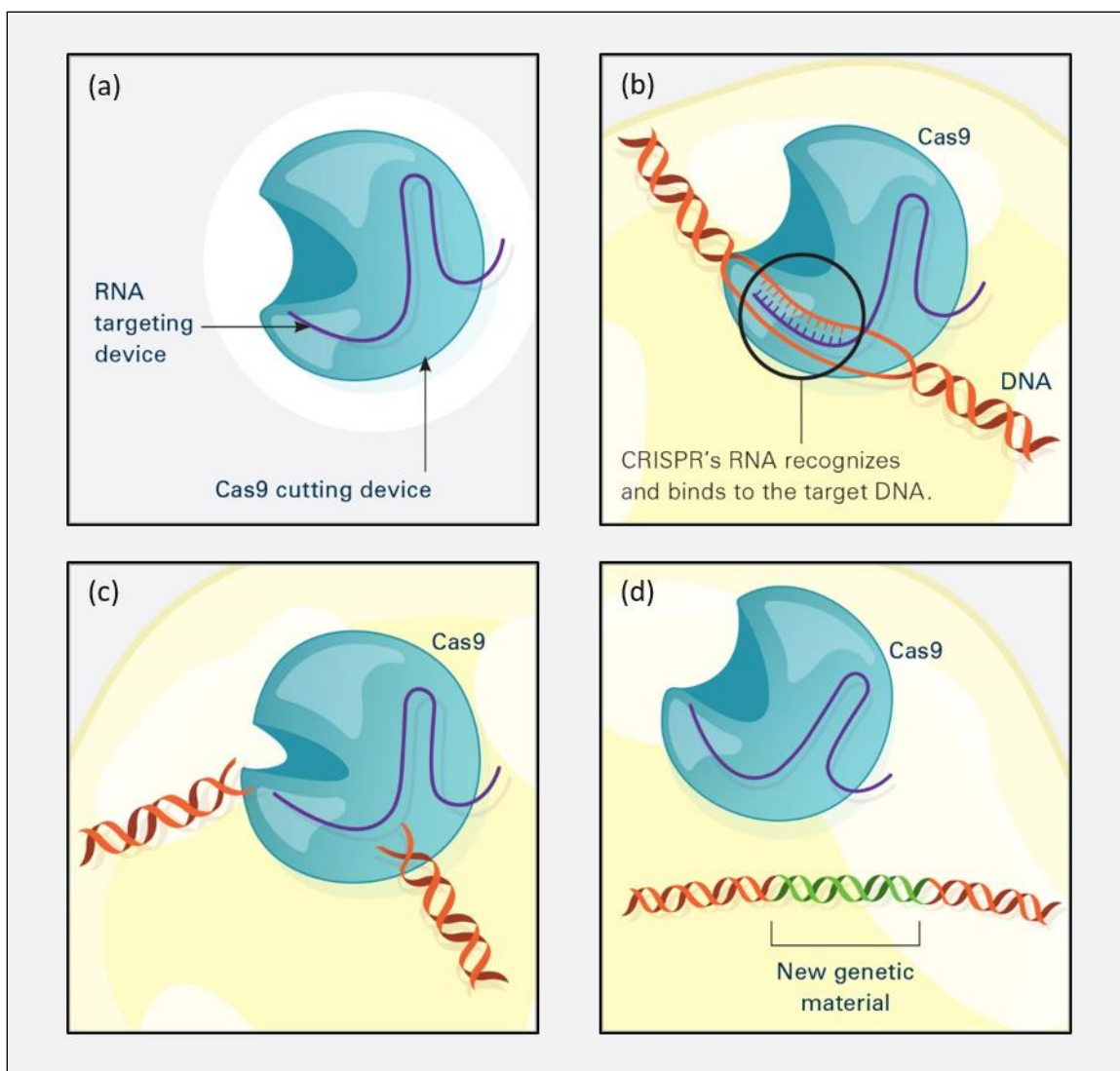
Figure 1. CRISPR-Cas9
