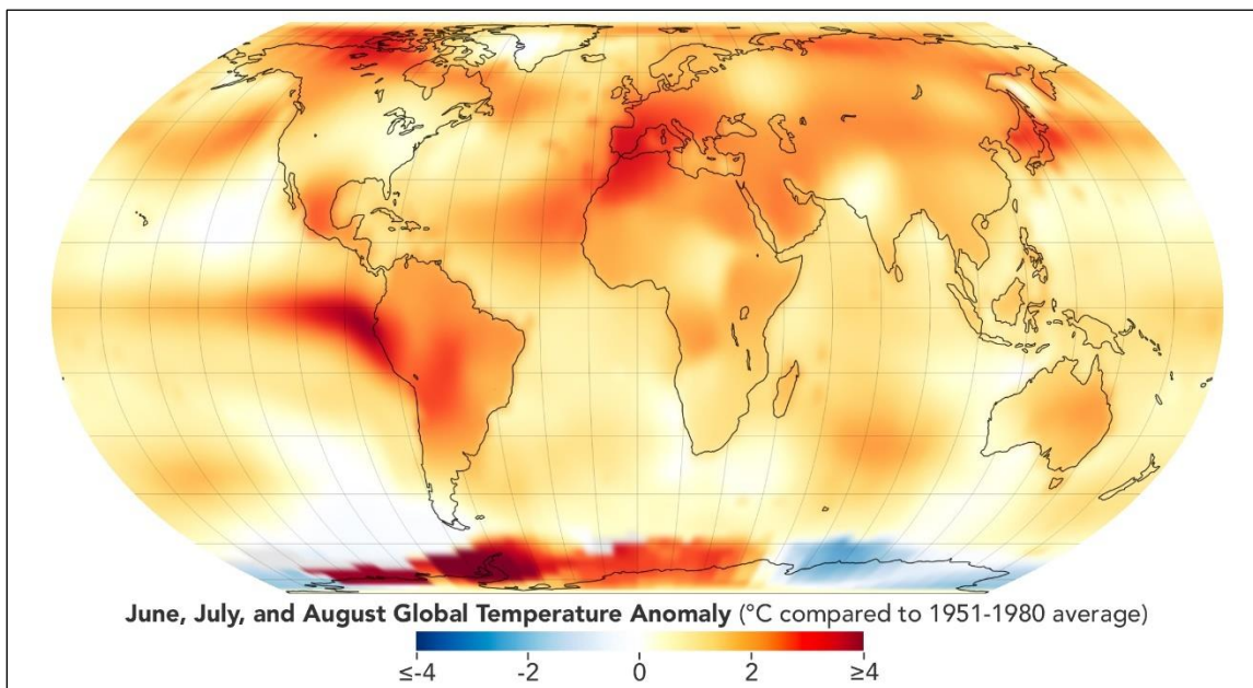
Figure 1. June, July, and August 2023 Global Temperature Anomaly
