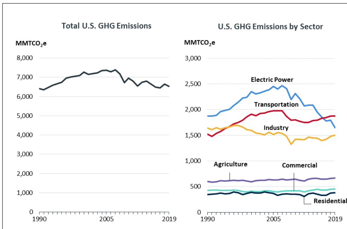
Figure I. U.S. GHG Emissions: 1990-2019
