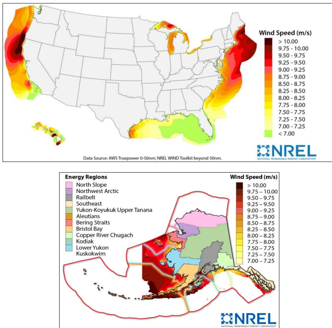
Figure 4. U.S. Offshore Wind Speed Estimates
