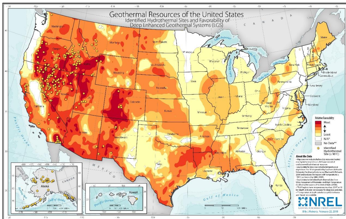
Figure 4. Hydrothermal Resources Identified in the United States
