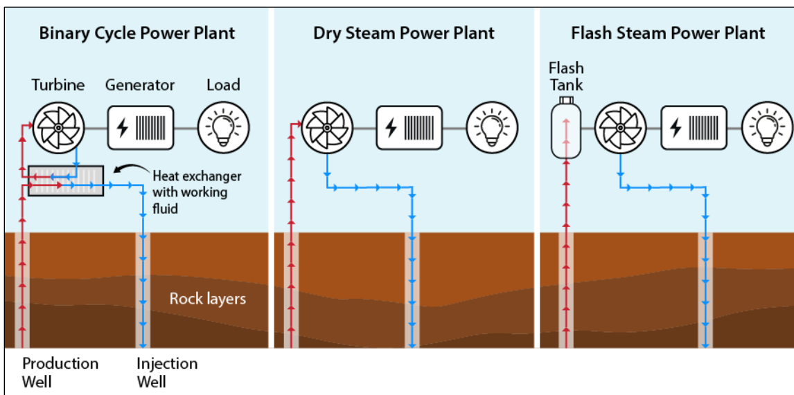
Figure 2. Three Primary Types of Geothermal Power Plants
