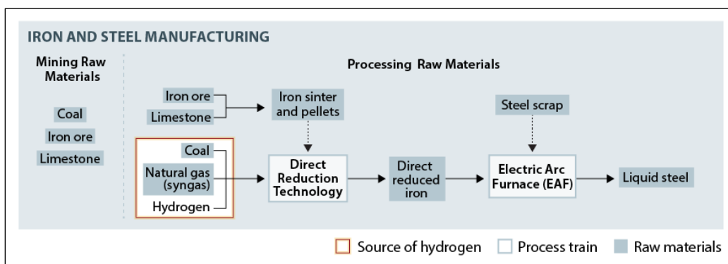
Figure 5. Direct Reduction of Iron
