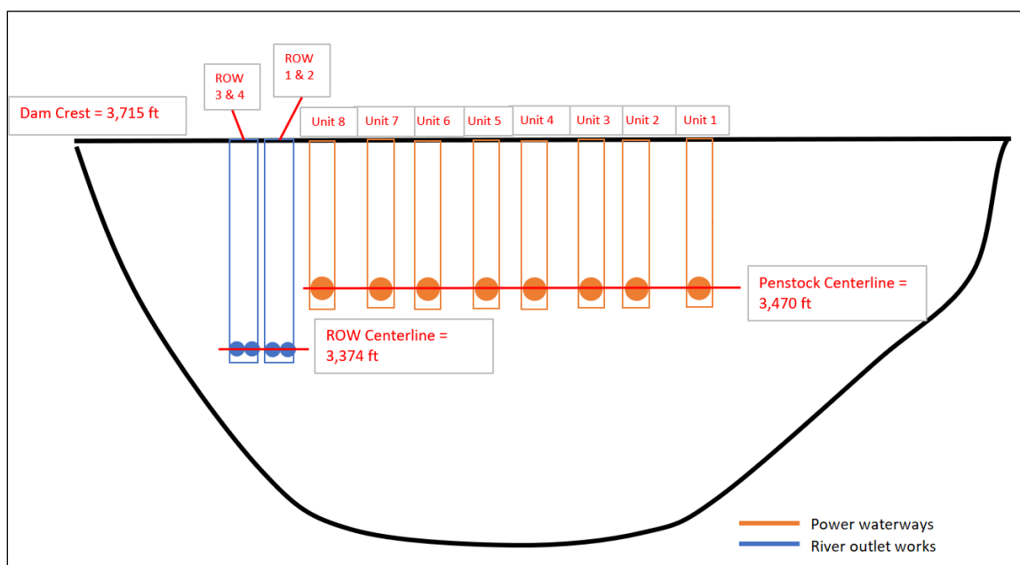
Figure 2. Glen Canyon Dam Outlet Elevations: Upstream View
