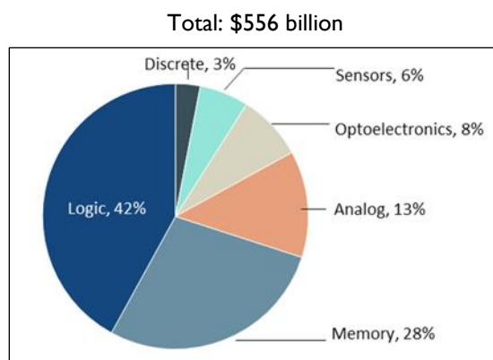
Figure 1. Semiconductor Sales, 2021
