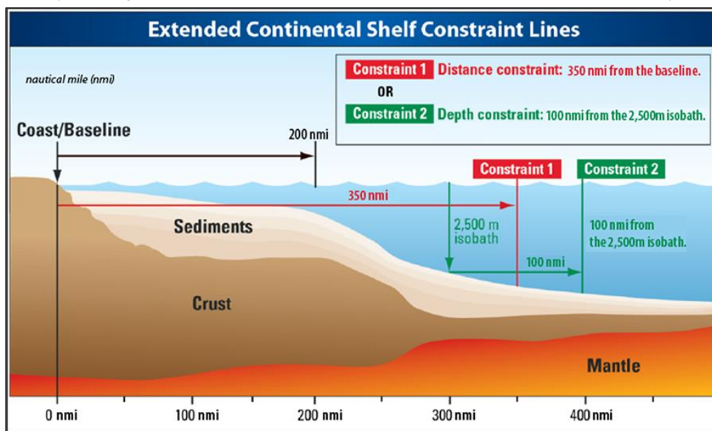
Figure 3. Constraints on the Extent of the Extended Continental Shelf
