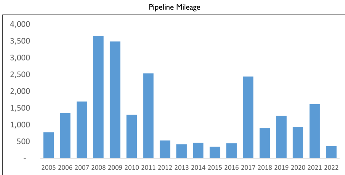
Figure 8. Annual U.S. Natural Gas Transmission Capacity Expansion and New Construction
