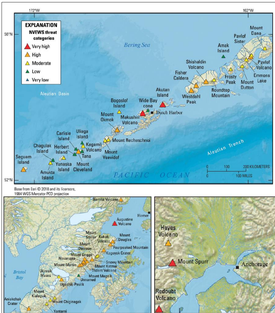
Figure 2. Detailed Maps of Some of the Highest Threat Volcanoes in Alaska
