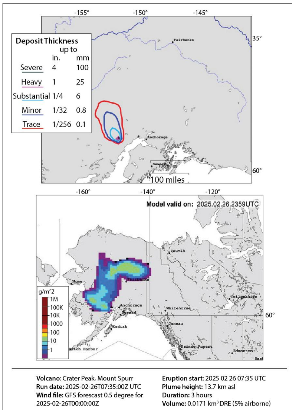
Figure 17. Models of Mount Spurr Ashfall and Ash Cloud Dispersion (February 26, 2025, eruption)
