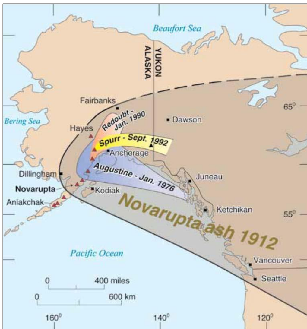
Figure 6. Extent of Ashfall From Some Major Alaskan Eruptions
