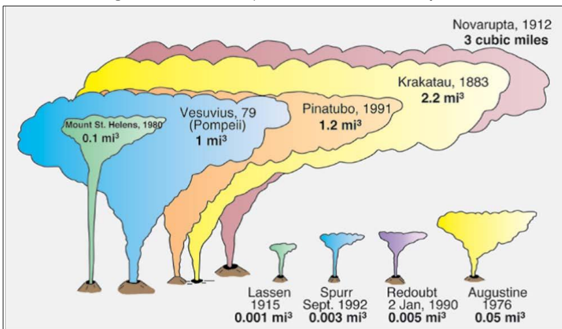
Figure 7. Volume of Major Alaskan and Other Eruptions
