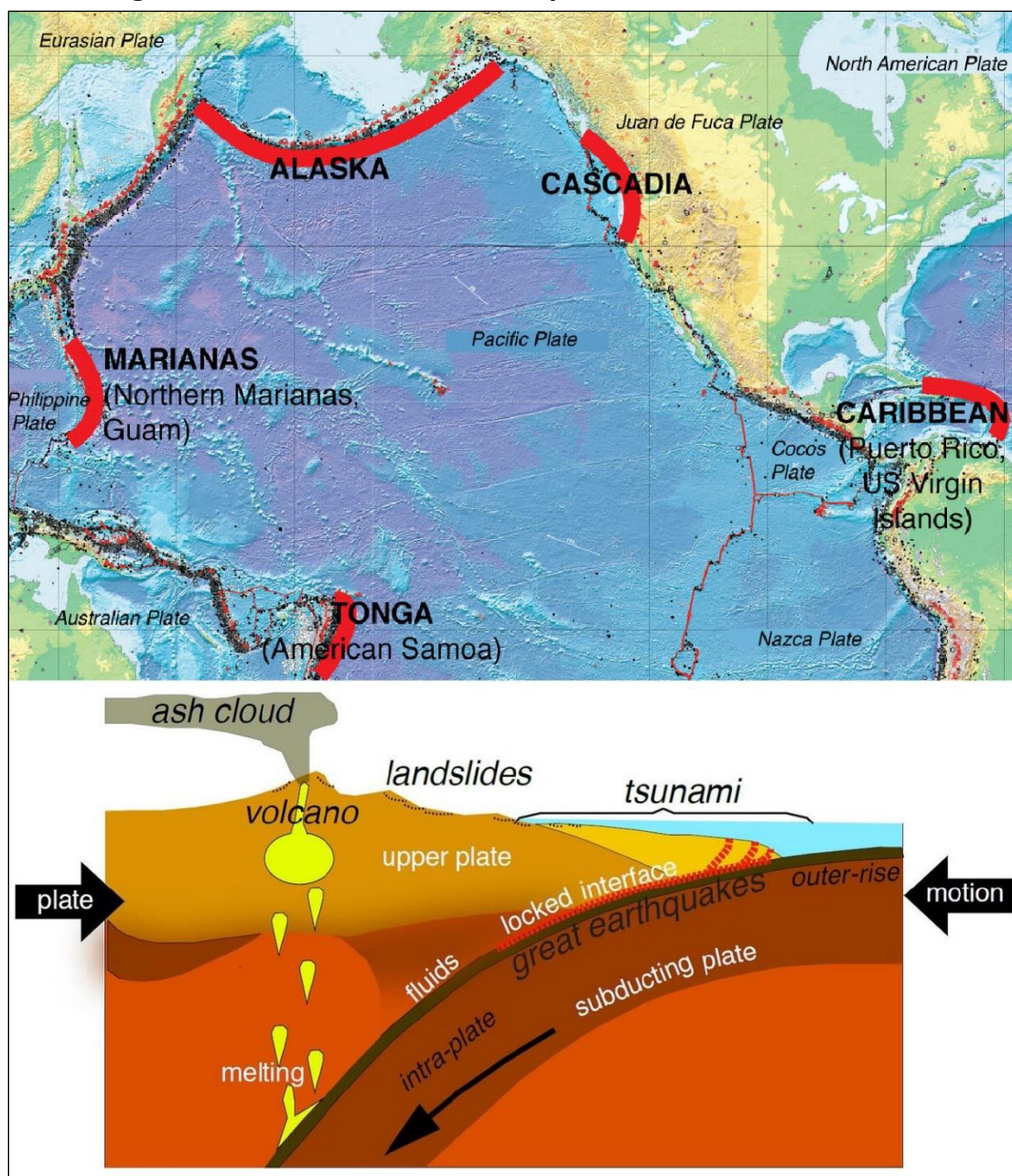
Figure 3. U.S. Subduction Zones Map and Subduction Zone Model
